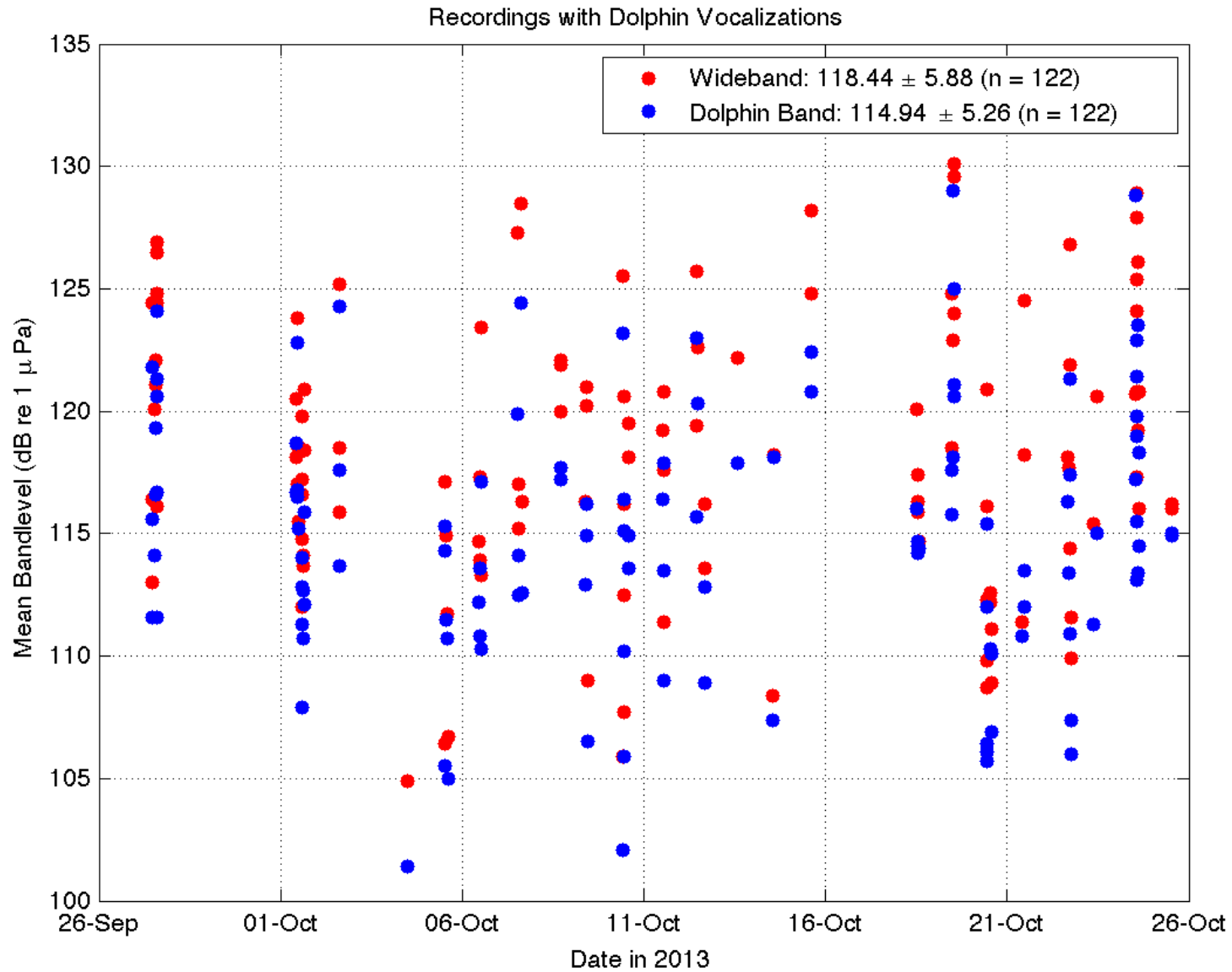
Figure 5.9 Mean bandlevels for the 122 recordings containing dolphin vocalizations. Bandlevels were analyzed in terms of both the 30–40,000 Hz “wideband” frequency range (red) and 400–12,500 Hz “dolphin-sensitive” band (blue).
